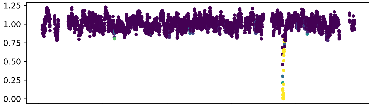
Single Model Predictions - KIC 11084727
