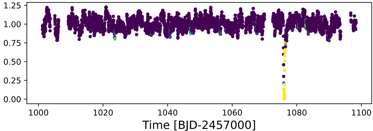
Single Model Predictions - KIC 11084727
